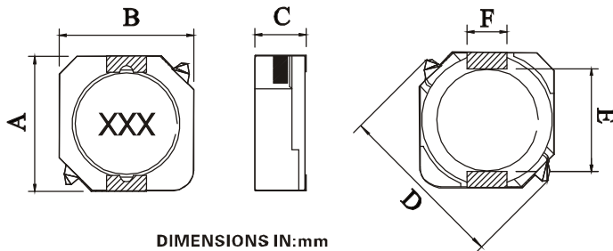
DIMENSIONS IN:mm
