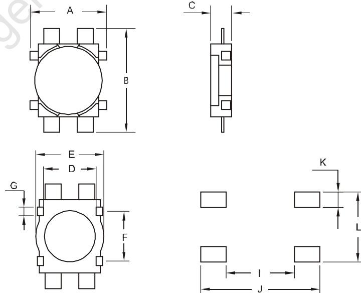
LAND PATTERNS
