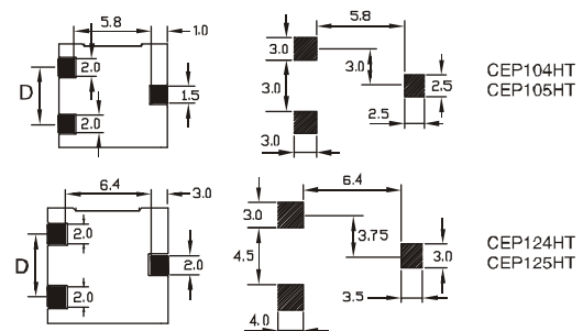
LAND PATTERN
