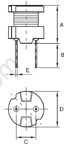
Dimension: mm
