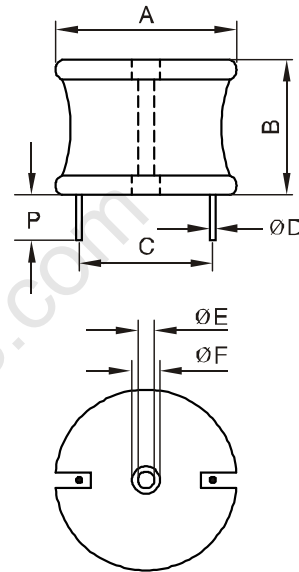
DIMENSIONS: inches/mm
