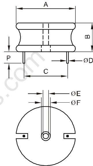
DIMENSIONS: inches/mm
